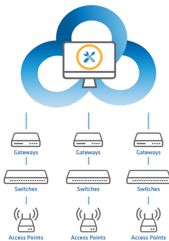
Fig. 2 Software-defined networking
