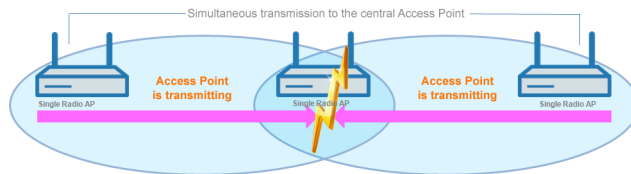
Figure 8: Simultaneous transmissions to the middle AP: The two outer APs are unaware of the collision.
