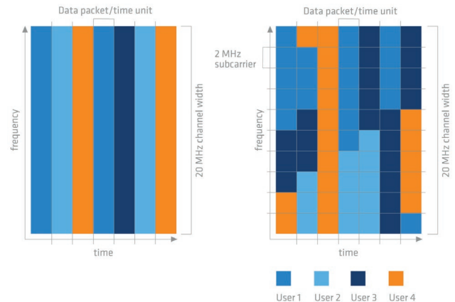
Fig. 3: Comparing OFDM vs. OFDMA technologies
