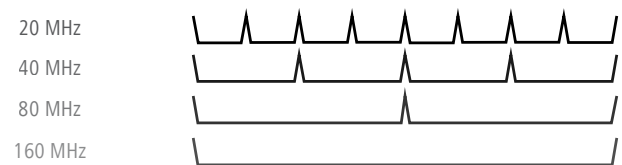
Fig. 1: Possible channel bandwidths with Wi-Fi 6
