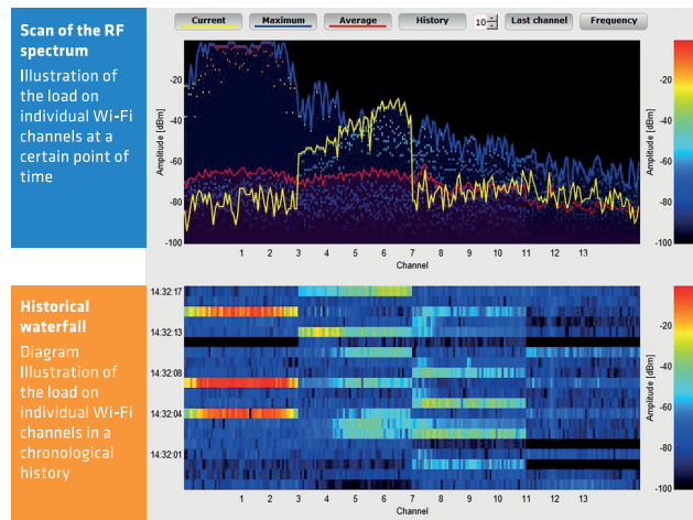
Fig. 8: Spectral Scan
