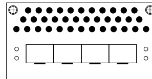
↓ LANCOM UF Extension Module 4× 10G SFP+ (UF-X60)
